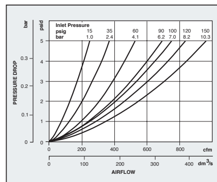
1-1/2" Pressure drop test
