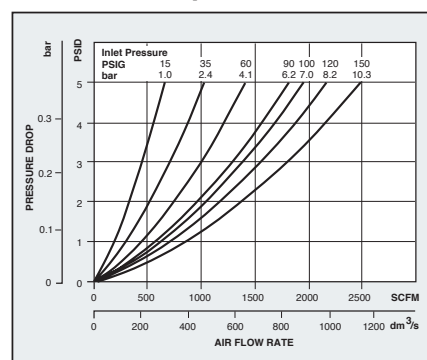
3" Pressure drop test
